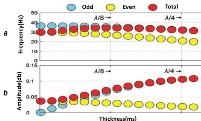
Fig. 2. Peak frequency and peak amplitude vs. thickness variation (modified after [4])
