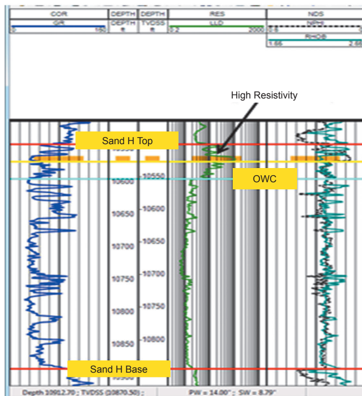
Fig. 15. Sands H in Otió-4 with high resistivity interpreted as hydrocarbon zones (Powerlog, 2014)
