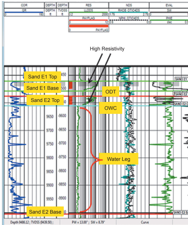
Fig. 14. Sands E1 and E2 in Otió-1 with high resistivity interpreted as hydrocarbon zones (Powerlog, 2014)
