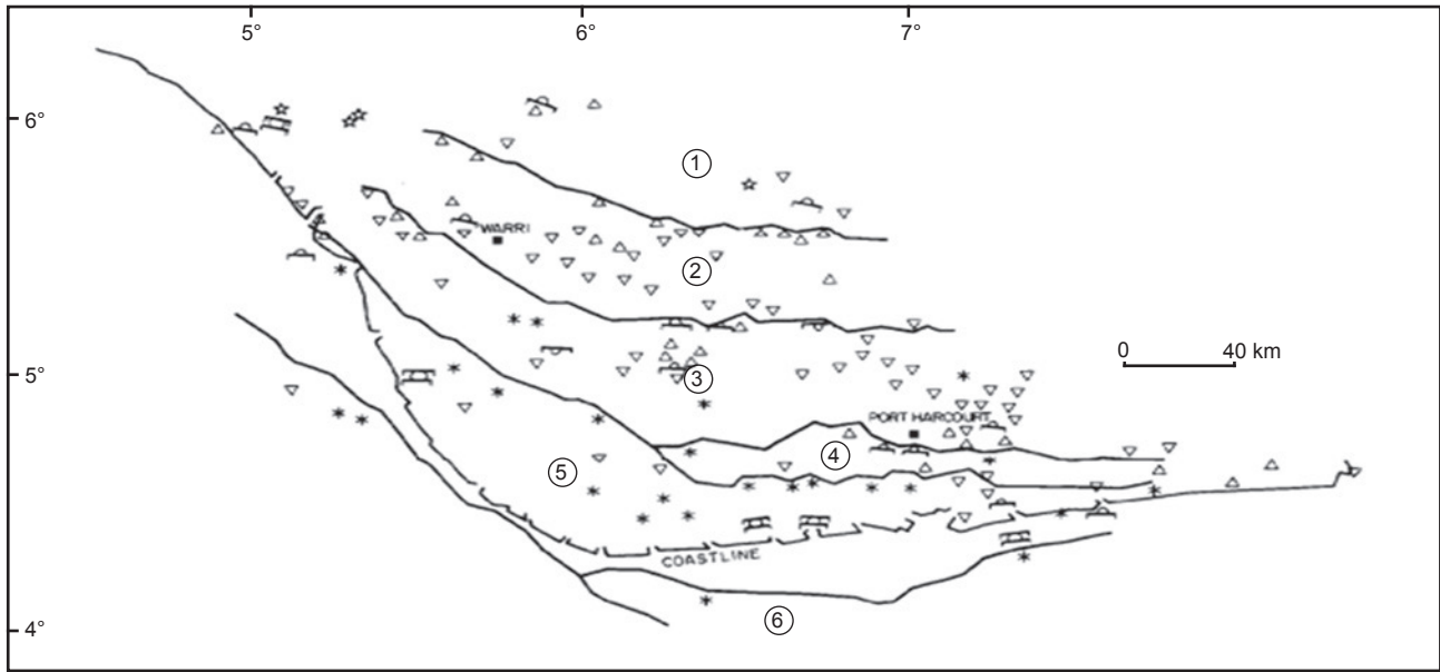
Fig. 3. Structural types of the Niger delta and associated depobelt [4]:
